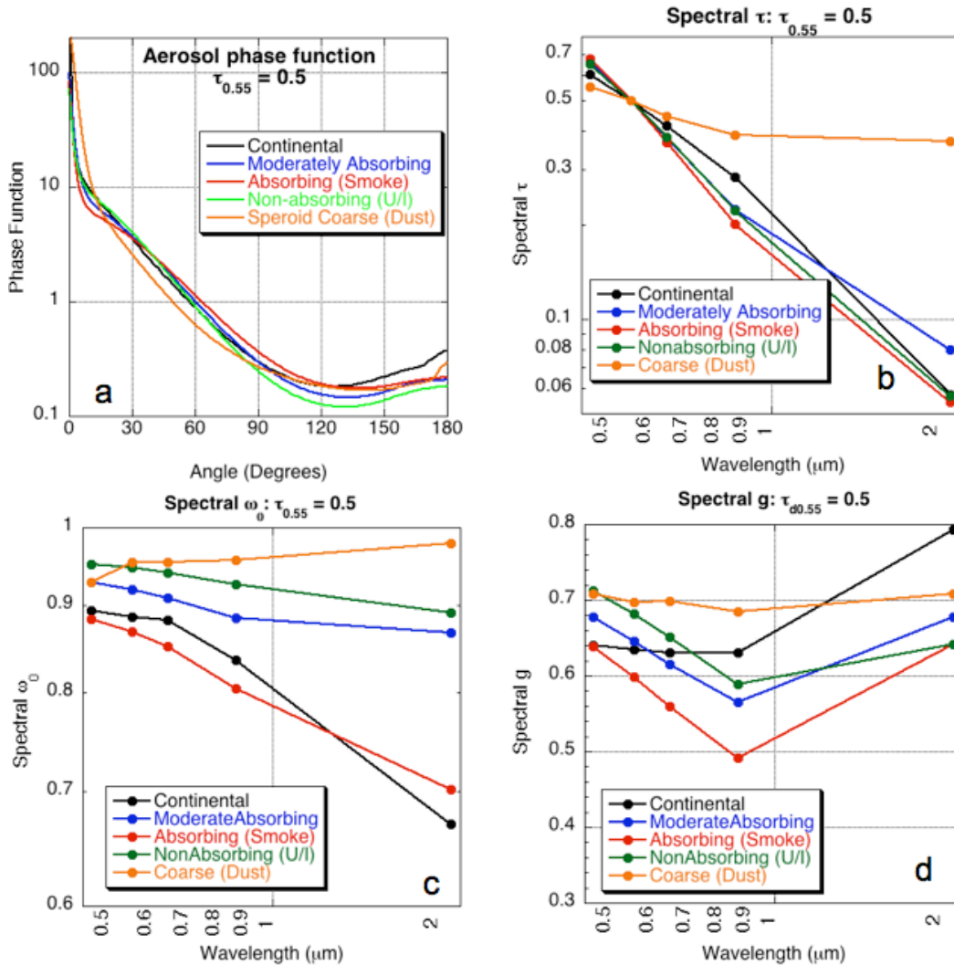
Figure 12: Plot of optical properties for the 5 aerosol models of the C005-L LUT, for \tau = 0.5 . a) phase function at 0.55 \mu\text{m} (as a function of angle) b) optical depth spectral dependence, c) single scattering albedo spectral dependence and d) asymmetry parameter spectral dependence.
