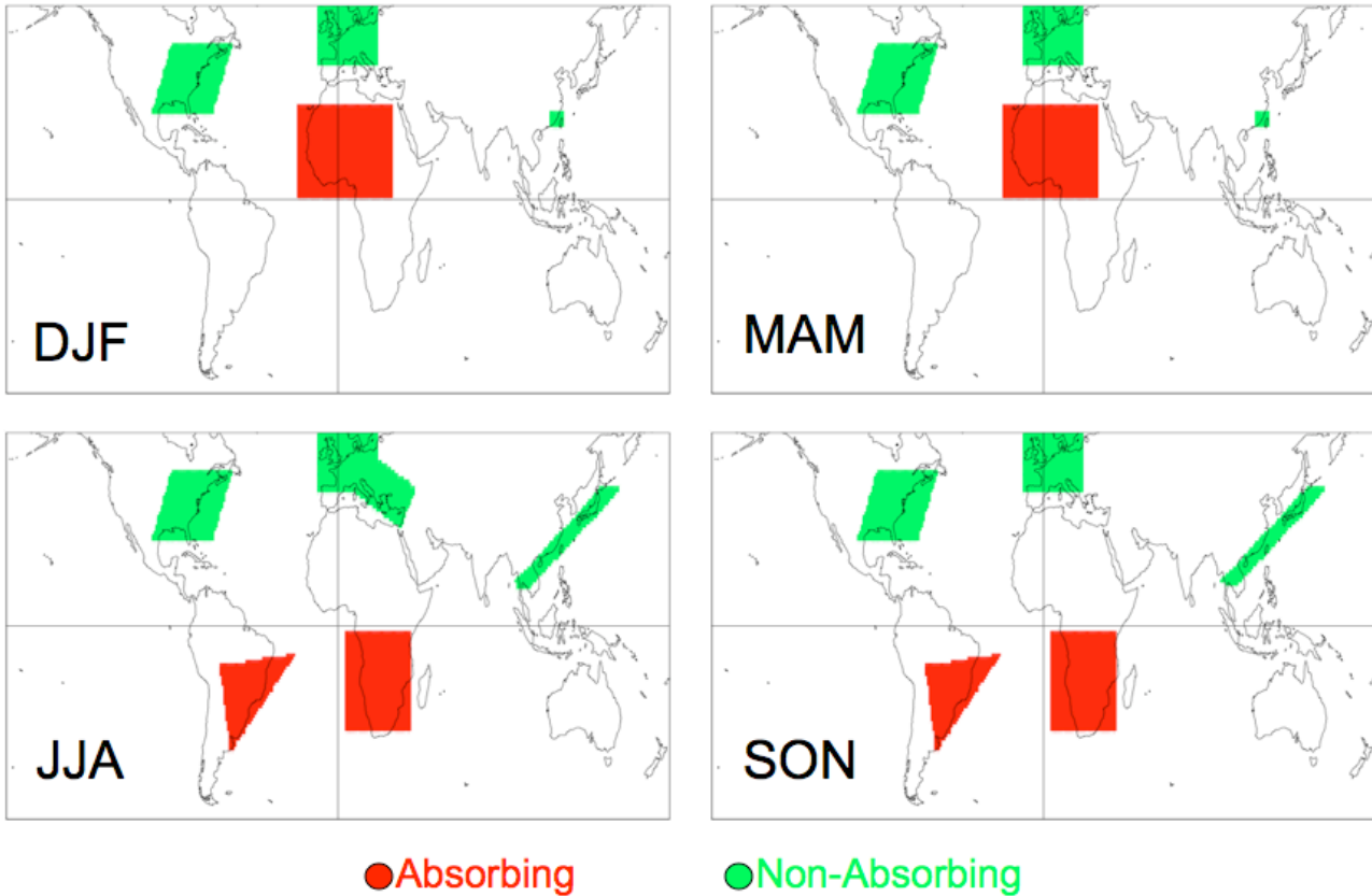
Figure 10: Final spherical aerosol model type designated at 1° x 1° gridbox per season. Red and green represent absorbing ( \omega_0 \sim 0.85 ) or non-absorbing ( \omega_0 \sim 0.95 ) models, respectively. Moderately absorbing ( \omega_0 \sim 0.90 ) is assumed everywhere else.
