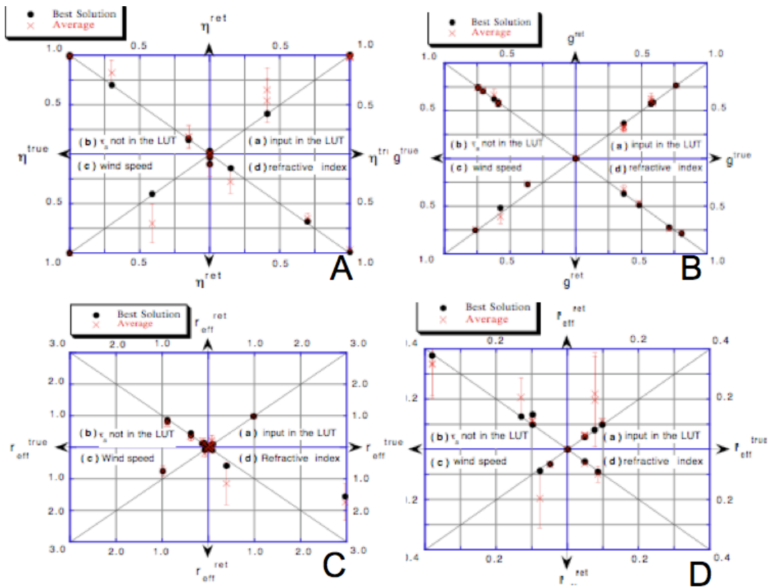
Figure 5: Same as Fig 4 but for (A) ratio \eta , (B) asymmetry parameter g , (C) Effective Radius ( R_{eff} ) and for (D) blowup of Effective Radius ( R_{eff} < 0.40 ). Error bars correspond to the standard deviation of the 'average' solution.
