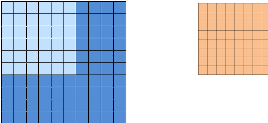
Figure 2. Product Sizes: At left: MODIS 10x10 km level 2 pixel retrieved from 1x1 km level 1b pixels, compared to the size of the VIIRS level 2 product size in lighter blue. At right: VIIRS 6x6km product retrieved from 0.75x0.75 km level 1b pixels.
