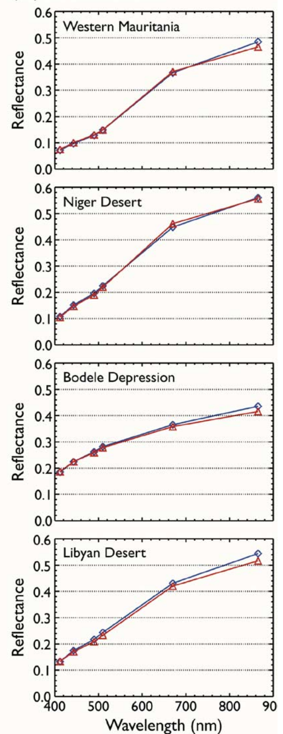
Fig. 5. (Left) Example of a precalculated land surface reflectivity database of 0.1^\circ latitude \times 0.1^\circ longitude resolution at 412- and 670-nm channels using 1-km SeaWiFS radiances for February 2000. Areas that do not have enough samples to achieve statistical significance due to persistent cloud cover are represented by white color. (Right) Spectral variations of surface reflectivity at six SeaWiFS channels from visible to near-infrared wavelengths for February 2000 (blue diamonds) and June 2000 (red triangles).
