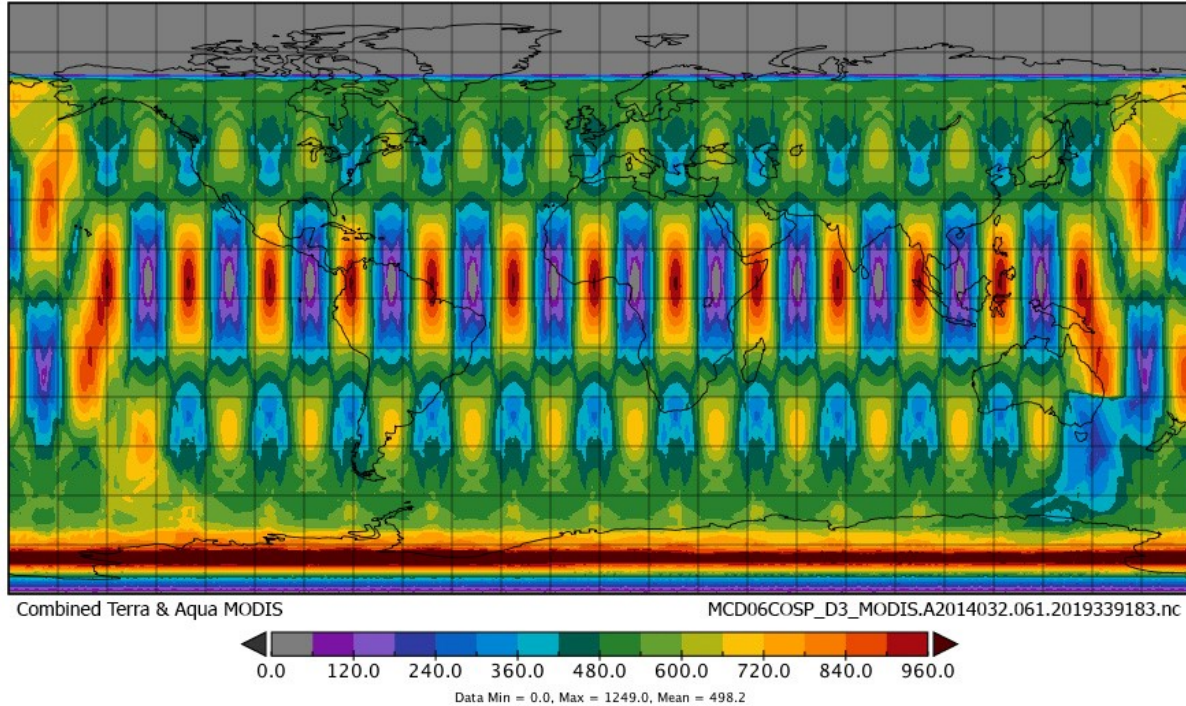
Figure 7. Global distribution of daily pixel counts for 1 Feb 2014 (i.e., the number of L2 data pixels per 1 \times 1^\circ L3 grid cell) for 1 \times 1 km resolution (sampled at 5km) L2 input products (where no aggregation is performed, limiting pixels) for MODIS Aqua + MODIS Terra. Note that this is a daytime only product. The date of this image is February 1, 2014 (same as the orbit track maps shown in Figure 6). The overlapping orbit tracks around the International Date Line (see the pattern breaks in that region) shows clearly the definition of day issue discussed in Section 1.3.
