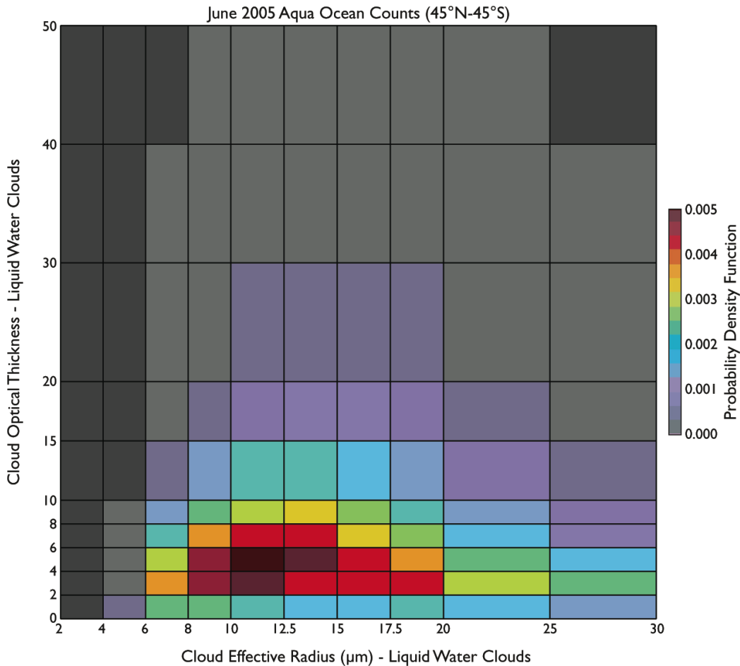
Figure 21. A June 2005 MYD08_M3 Normalized Probability Density Function (PDF) Joint Histogram of Cloud Optical Thickness (y-axis) vs. Cloud Effective Radius (x-axis) for Liquid Water Clouds displayed as a “colored histogram bin plot” with post-processing to limit the data to Ocean-only L3 grid cells that range from 45N to 45S. The top bin of Cloud Optical Thickness from 50 to 100 was removed. The bin colors represent the PDF in each bin (low probability is grey, high probability is red).
