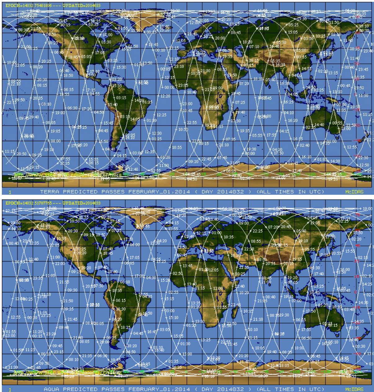
Figure 6. Predicted Terra MODIS orbit tracks (top), and Predicted Aqua MODIS orbit tracks (bottom), for a particular day (February 1, 2014).
