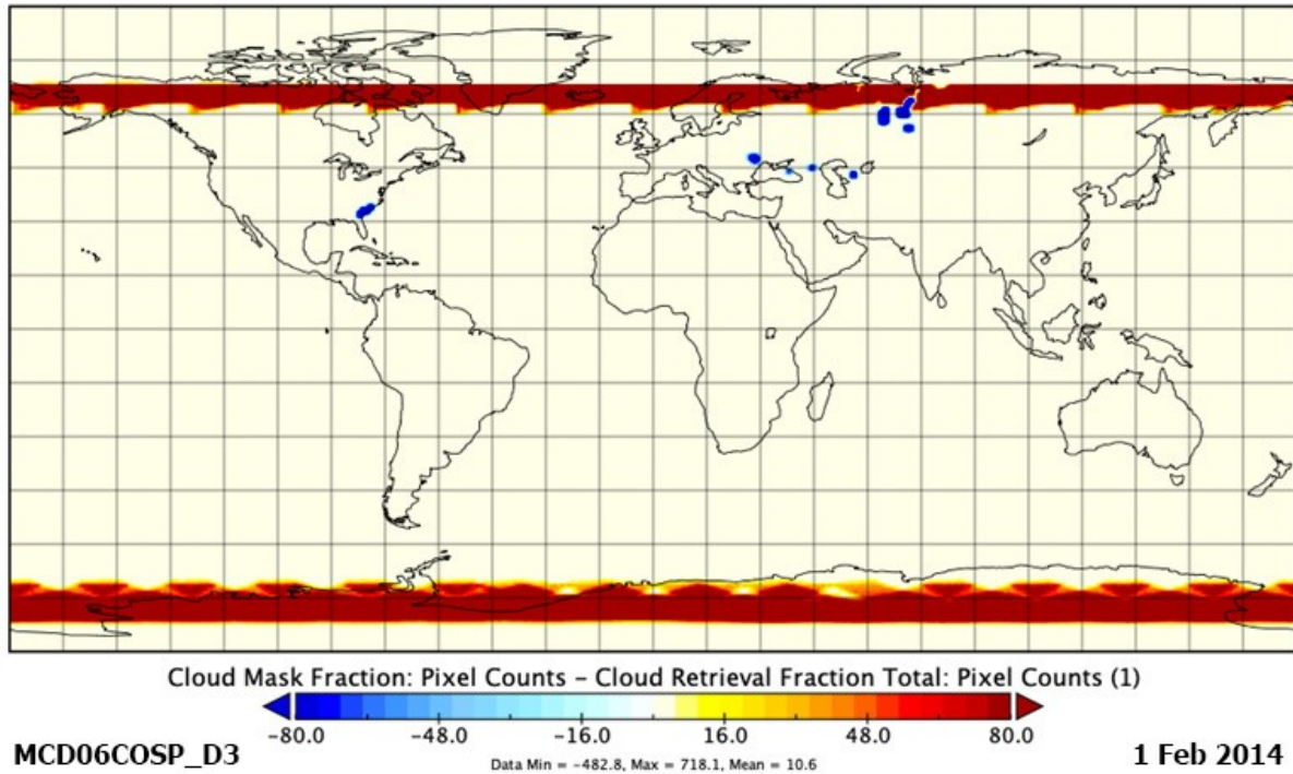
Figure 13. A depiction of the pixel count differences (Cloud_Mask_Fraction - Cloud_Retrieval_Fraction_Total) in the MCD06COSP_D3 file for 1 Feb 2014. The blue color on the image (corresponding to negative difference values) shows regions impacted by the Cloud Top Property bug, where intermittent missing values produced lower pixel counts of Cloud_Mask_Fraction. It should be noted that the actual mean or mean fraction values did not show any visible impact, only the pixel count statistic showed visible impact. As a final note, the red colored areas towards the polar regions are normal (expected), and show where the Cloud Top Property retrieval algorithm retrieved farther poleward than the Cloud Optical Property algorithm (due to differing definitions of the extent of daytime or sunlit scenes in these two retrieval algorithms). The 0 count regions on the poleward side of these red colored bands are technically fill data since this is a daytime only product -- but for the pixel count statistic, fill data is recorded as 0 counts.
