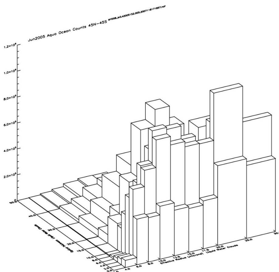
Figure 18. A June 2005 MYD08_M3 Counts Joint Histogram of cloud optical thickness (y-axis) vs. cloud effective radius (x-axis) for liquid water clouds displayed as a “3D lego plot” with post-processing to limit the data to ocean-only L3 grid cells that range from 45°N to 45°S. The top bin of cloud optical thickness from 50 to 100 was chopped off. The height of each Lego bar represents the number of counts in each bin. Orienting all bins to render lego plots visible is often difficult to impossible.
