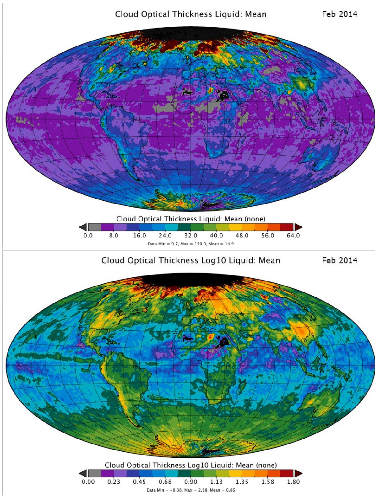
Figure 12. L3 COSP (Terra MODIS + Aqua MODIS) Monthly Images for Feb 2014 (a) Cloud Optical Thickness for Liquid Water Phase Clouds (full valid range from 0.01 to 150.0) (b) The Logarithm (Log) of that exact same data (full valid range from -2.0 to 2.176). Note the image scale ranges were tweaked on both images to provide more detail.
