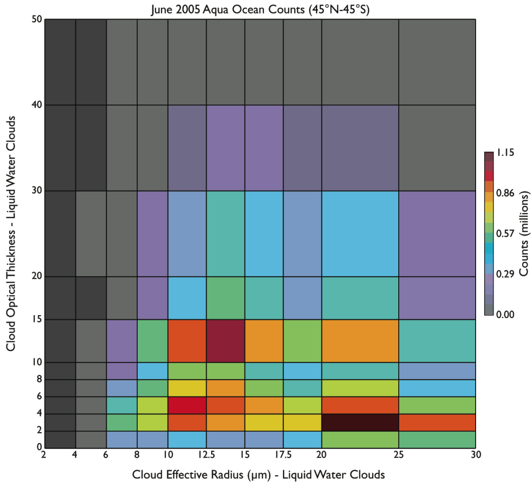
Figure 20. A June 2005 MYD08_M3 Counts Joint Histogram of cloud optical thickness (y-axis) vs. cloud effective radius (x-axis) for liquid water clouds displayed as a “colored histogram bin plot” with post-processing to limit the data to ocean-only L3 grid cells that range from 45°N to 45°S. The top bin of cloud optical thickness from 50 to 100 was chopped off. The bin colors represent the number of counts in each bin (low is grey, high is red).
